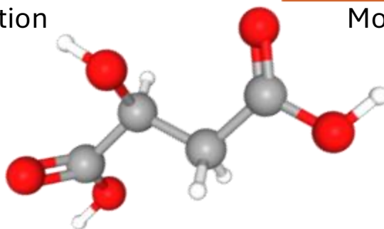
Malic acid molecule (Ball-and-stick model)
